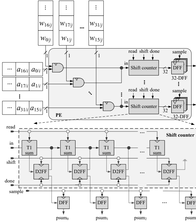
Figure 10. The proposed SFQ-based 16-bit bit-serial PE with OS dataflow, where the Shift counter circuit is designed for partial products accumulation.
