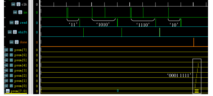
Figure 11. Simulation result of the Shift counter.
