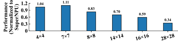
Figure 13. JB-SA's performance with various spatial sizes of the ofmap tile, normalized to SuperNPU.
