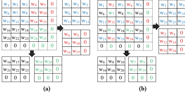
Figure 15. The partition of a 5 \times 5 convolutional kernel using (a) stride = 1 and (b) stride = 2, respectively.
