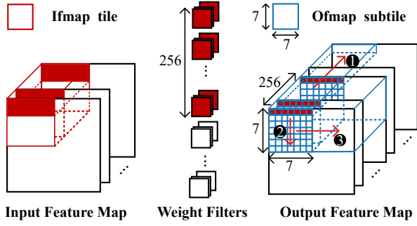
Figure 12. Data partitioning and scheduling of the convolutional layer.
