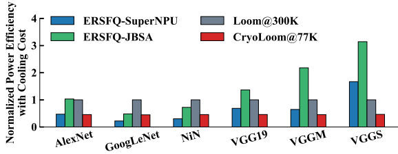
Figure 21. Power efficiency comparison of ERSFQ-based JBSA, ERSFQ-based SuperNPU, Loom@300K, and CryoLoom@77K considering cooling cost, normalized to Loom@300K.
