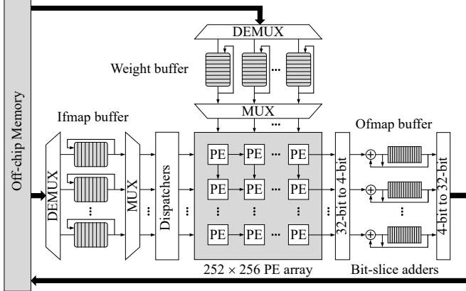
Figure 9. The overview of JBSA.
