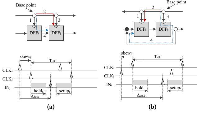
Figure 3. Typical SFQ clocking schemes: (a) concurrent-flow clocking, and (b) counter-flow clocking modified from [12].
