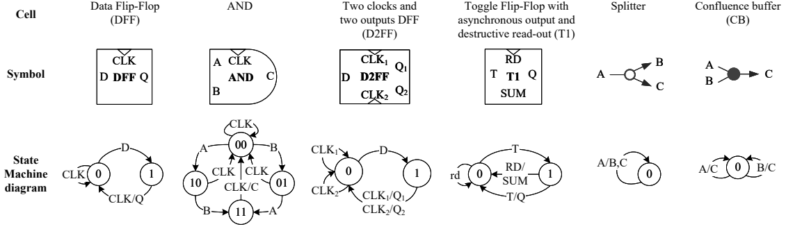
Figure 2. Symbols and state machine diagrams of fundamental SFQ gates: DFF, AND, D2FF, T1, splitter, and confluence buffer.
