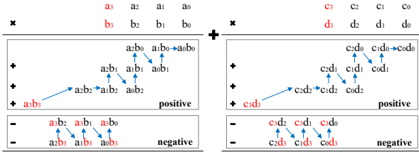
Figure 4. Example of bit-serial MAC operation: A \cdot B + C \cdot D , where A, B, C, and D are 4-bit signed numbers with a_3, b_3, c_3, and d_3 as sign bits.
