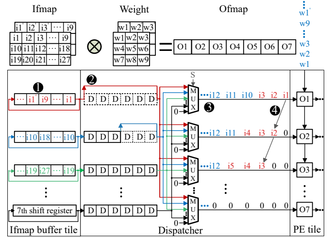
Figure 14. Dispatcher with a working example.
