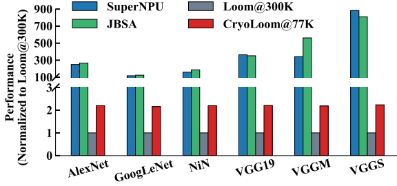
Figure 17. Normalized performance comparison of JBSA, SuperNPU, Loom@300K, and CryoLoom@77K.
