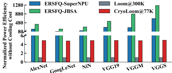
Figure 20. Power efficiency comparison of ERSFQ-based JBSA, ERSFQ-based SuperNPU, Loom@300K, and CryoLoom@77K considering no cooling cost, normalized to Loom@300K.
