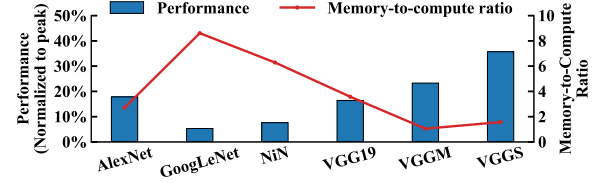
Figure 5. SuperNPU's performance (normalized to its peak performance) and the ratio of memory access time to computation time.
