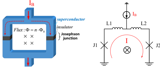
Figure 1. Superconducting ring with Josephson junctions and its equivalent circuit.
