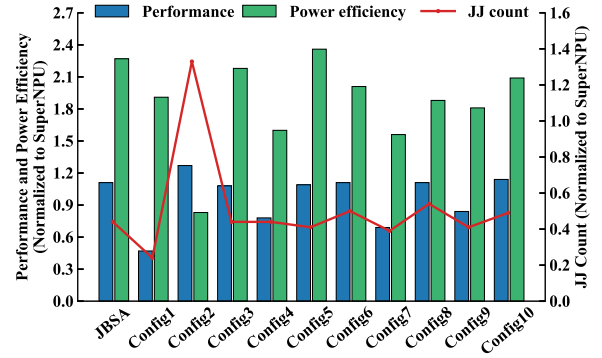
Figure 16. Performance, power efficiency and JJ count comparison of different architectural configurations for SFQ-based bit-serial DNN accelerators.
